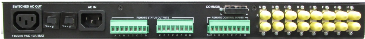
8:1 Rear Panel Shown Above (ST network ports)
